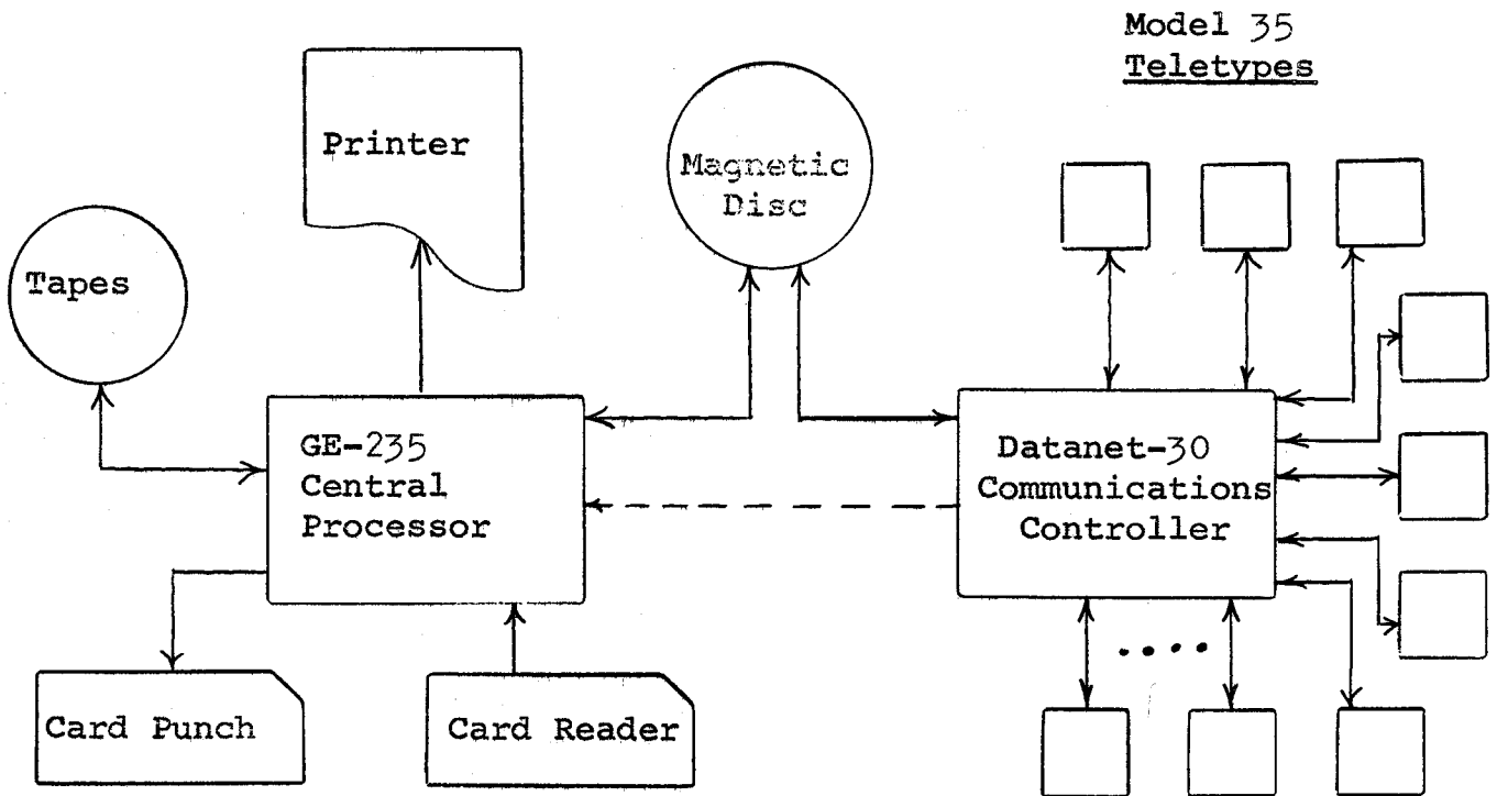
Schematic Diagram of System Hardware
